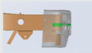
Front Bumper with Integrated FUPD
